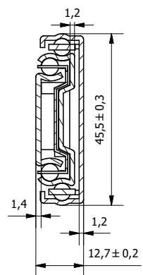
C-C (1:1)
